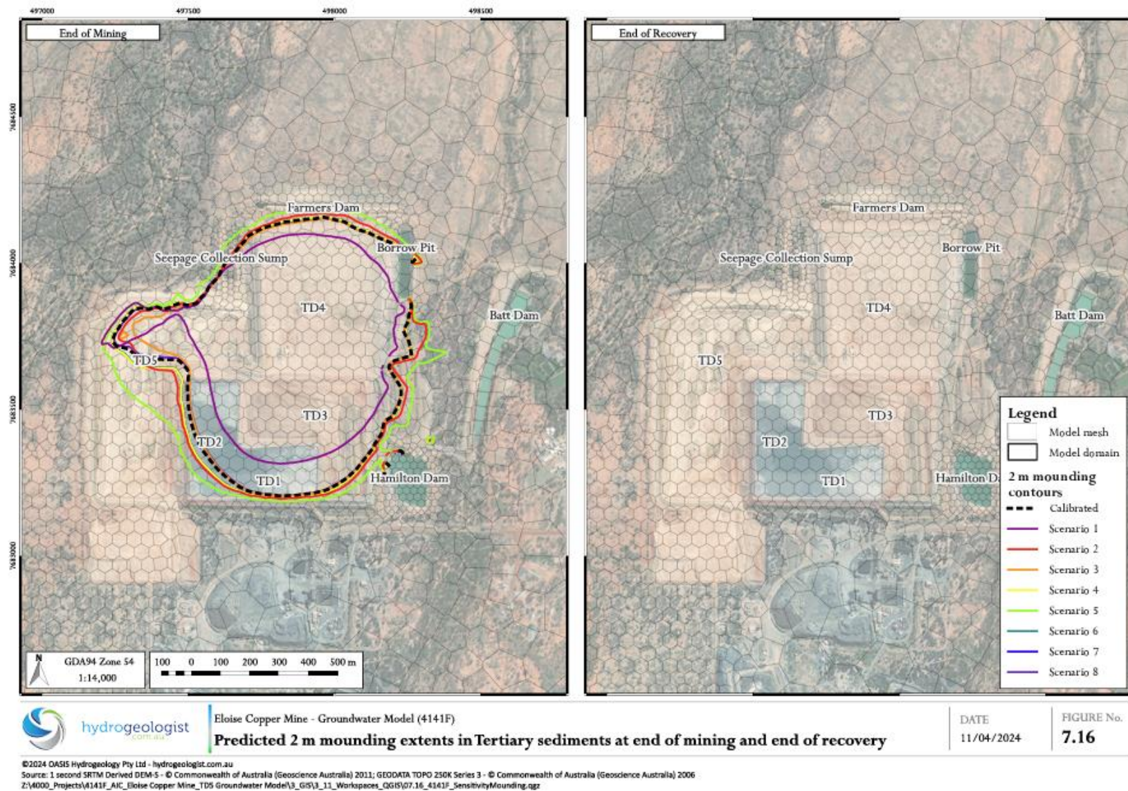
Figure 4: Groundwater mounding
